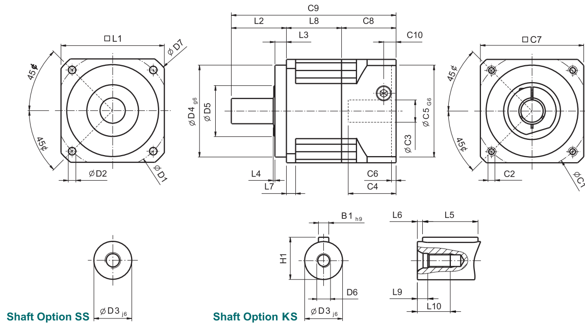
Shaft Option SS
