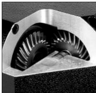
Spiral Bevel gear design
