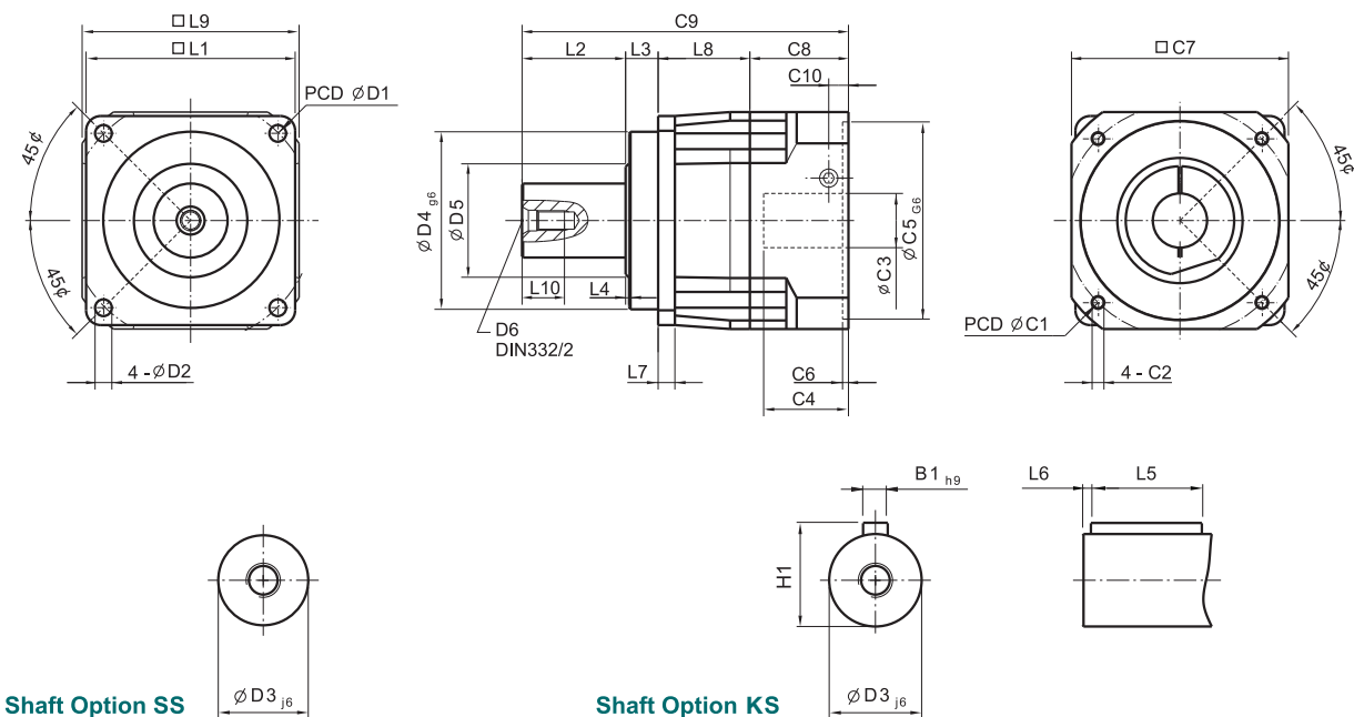
Shaft Option SS
